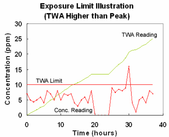
Figure 2. TWA can exceed the Peak value if readings are accumulated for more than 8 hours.
